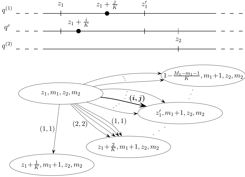
Figure 2: A section of a multiple description scalar quantizer and the corresponding graph.
